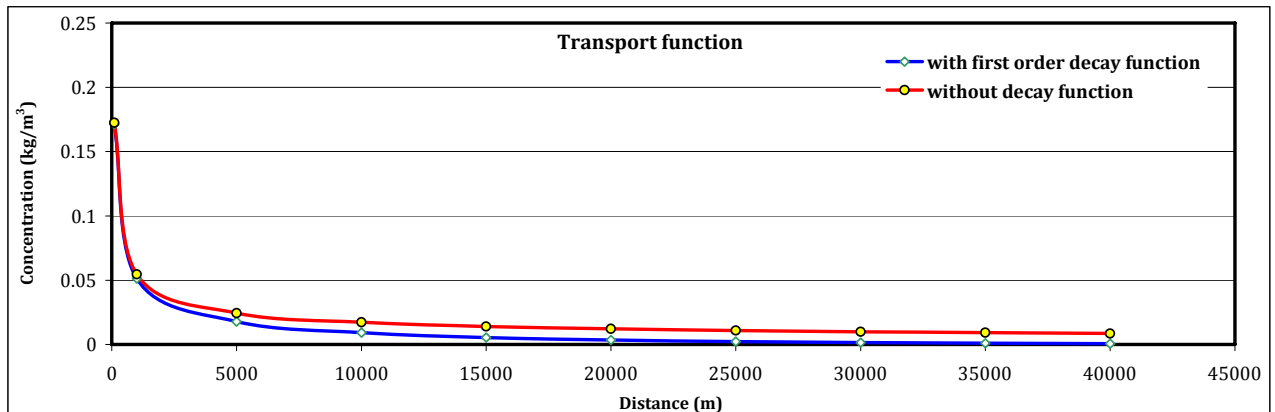
Fig. 9: Illustration to calculate the maximum concentration as a function of distance.
