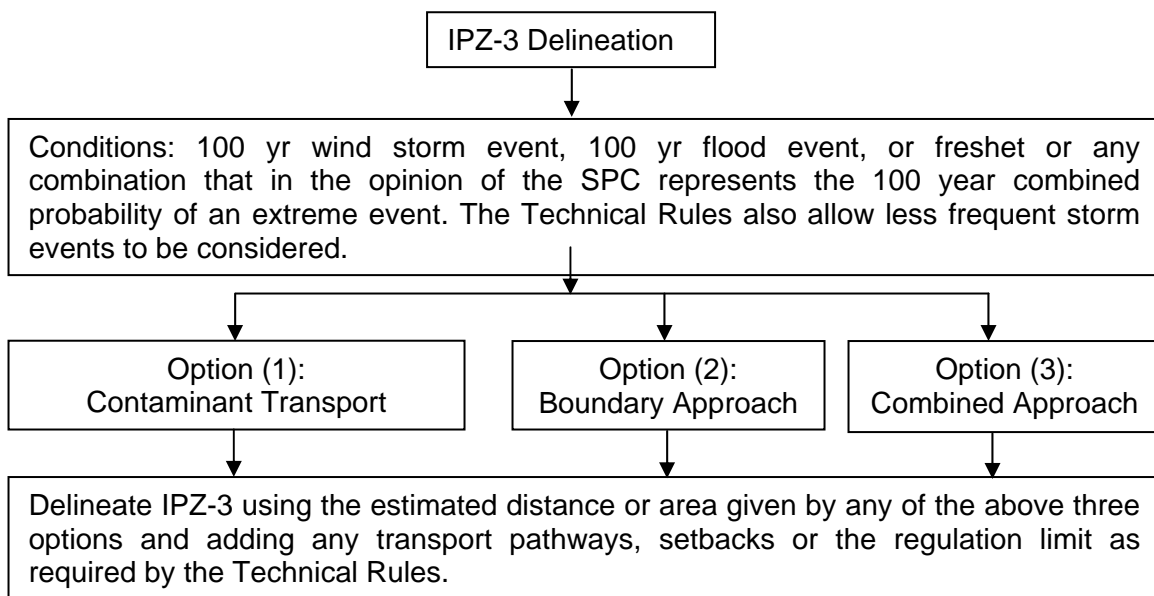
Fig. 1: Flowchart on options used for delineating IPZ-3.
